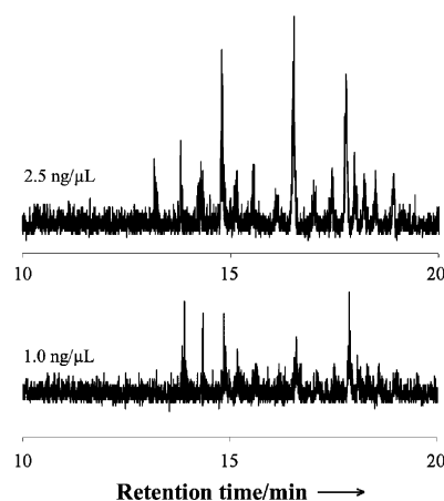
Figure 4. DNA separation by BaNC-HDC at single-molecule level. The separation capillary had a total length of 40 cm length (35 cm effective). The injection volume was estimated to be 2.4 pL. The elution pressure was 0.69 MPa. The values above the chromatograms represent the total DNA concentration. All other conditions were as in Figure 2A.
